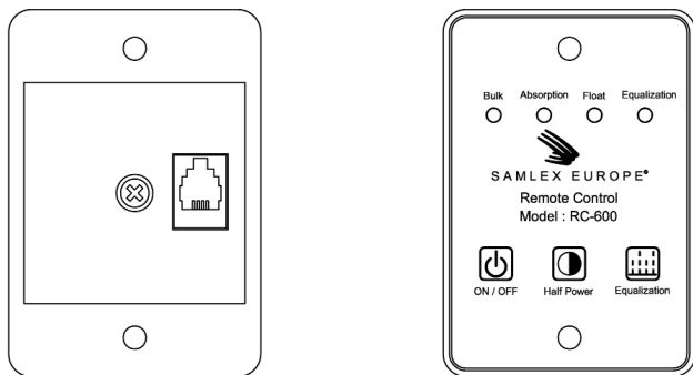
Figura 10 Control remoto RC-600
